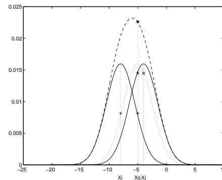
227 Fig. 1. One kernel at x_s ( dotted kernel ) or two kernels at x_i and x_j ( left and right ) 228 lead to the same summed estimate at x_s . This shows a figure consisting of different 229 types of lines. Elements of the figure described in the caption should be set in italics, 230 in parentheses, as shown in this sample caption. The last sentence of a figure caption 231 should generally end without a full stop 231 232 233 234 235 236 237 238 239 240 241 242 243 244 245
