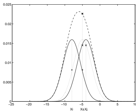
176 Fig. 1. One kernel at x_s ( dotted kernel ) or two kernels at x_i and x_j ( left and right ) 177 lead to the same summed estimate at x_s . This shows a figure consisting of different 178 types of lines. Elements of the figure described in the caption should be set in italics, 179 in parentheses, as shown in this sample caption. The last sentence of a figure caption 180 should generally end without a full stop
